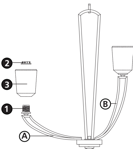
Drawing 2 - Fixture Assembly
