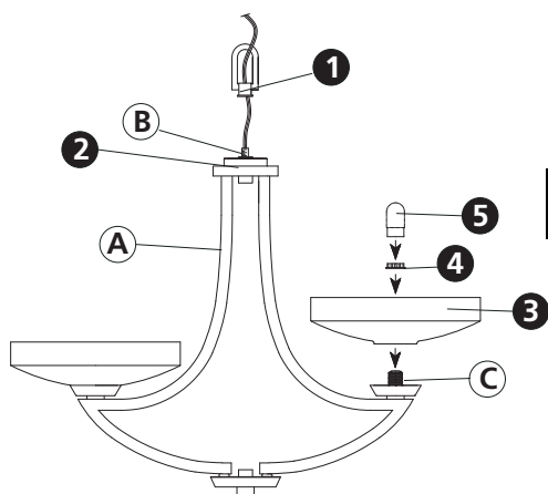
Drawing 2 - Fixture Assembly
