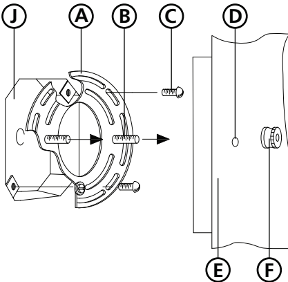
Drawing 1 - Fixture Mounting
