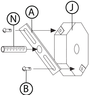
Drawing 2 - Mounting Assembly
